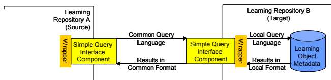
Figura 1. API SQI: Simple Query Interface
